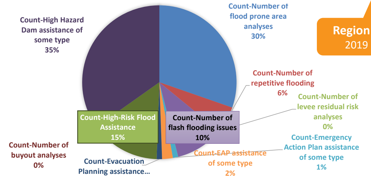
DISTRIBUTION OF THE COUNT OF FLOOD MITIGATION ACTIONS BY TYPES REGION K LHMP, 2019
